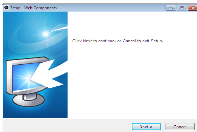
Figure 3-3 Plug-in-Installation (1)
