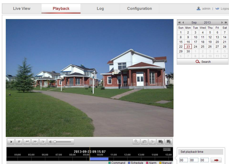
Figure 10-1 Wiedergabedialog
