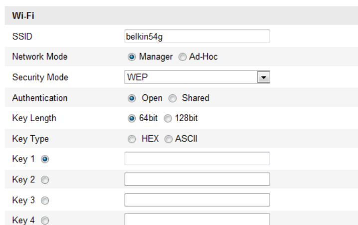
Figure 4-7 WEP-Modus
