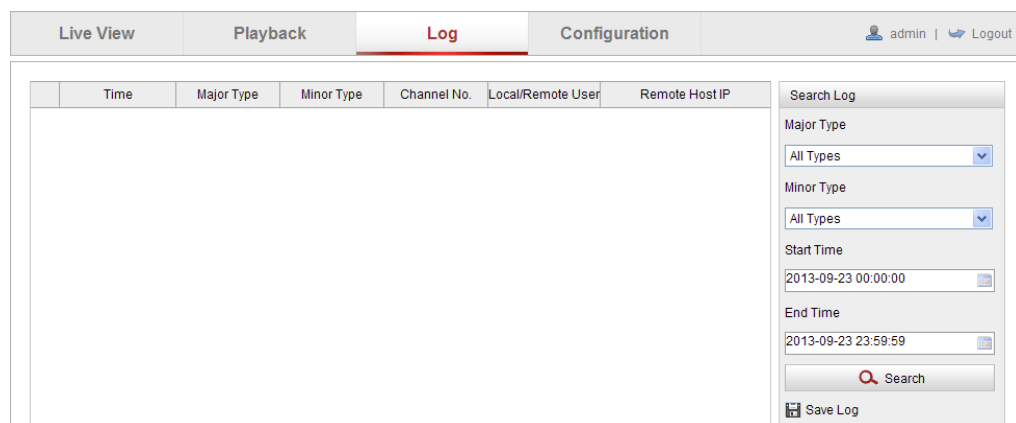
Figure 11-1 Protokollsuchdialog
