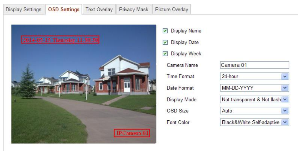
Figure 6-38 OSD-Einstellungen
