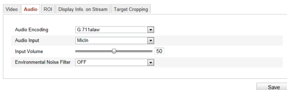
Figure 6-30 Audioeinstellungen
