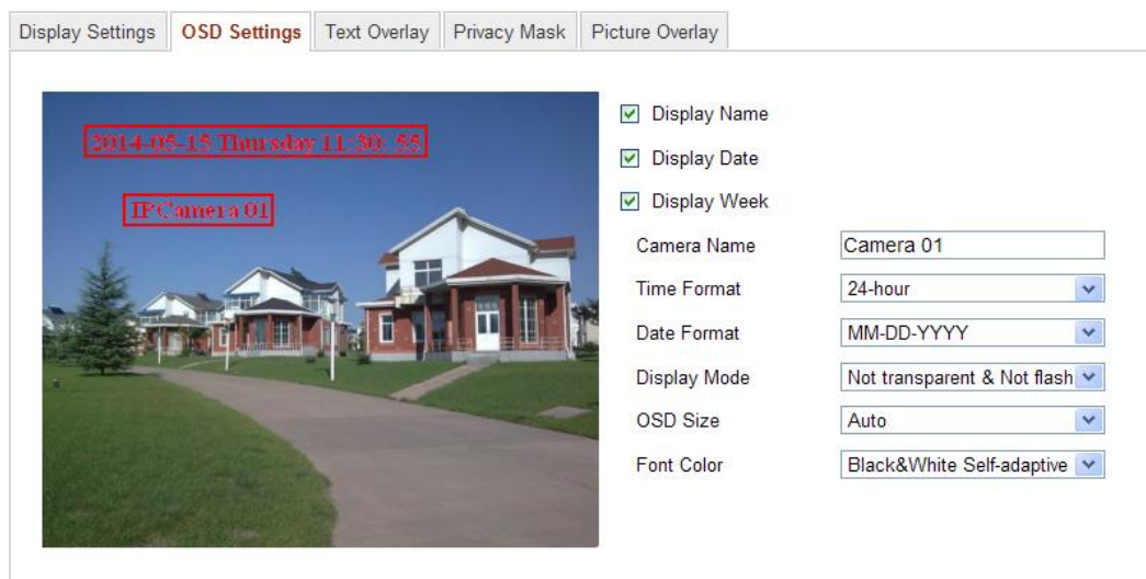
Figure 6-40 OSD-Lage anpassen
