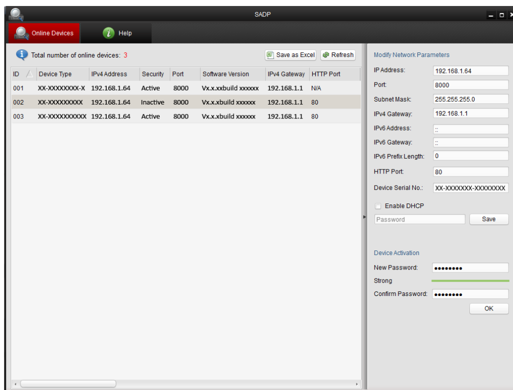
Figure 2-4 SADP-Schnittstelle
