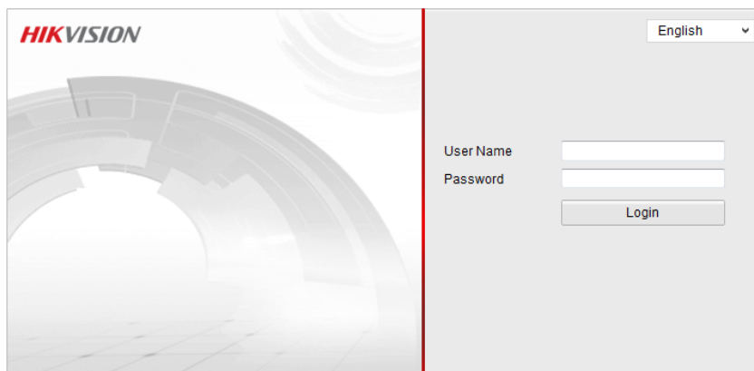
Figure 3-1 Anmeldedialog
